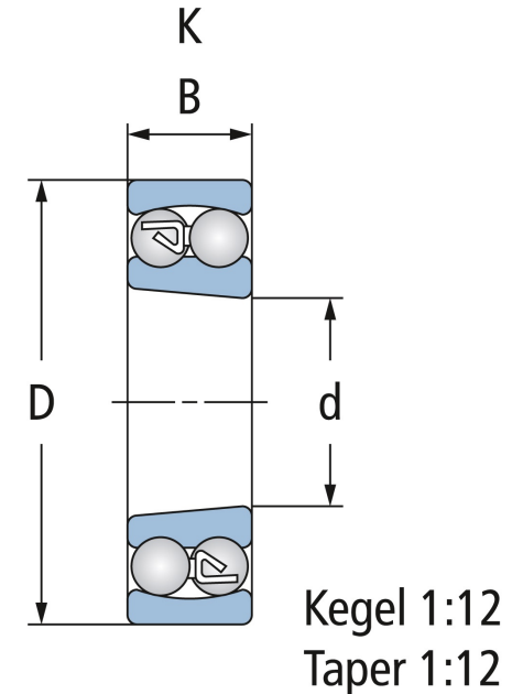
Kegelige Bohrung Tapered bore Kegel 1:12 Taper 1:12
